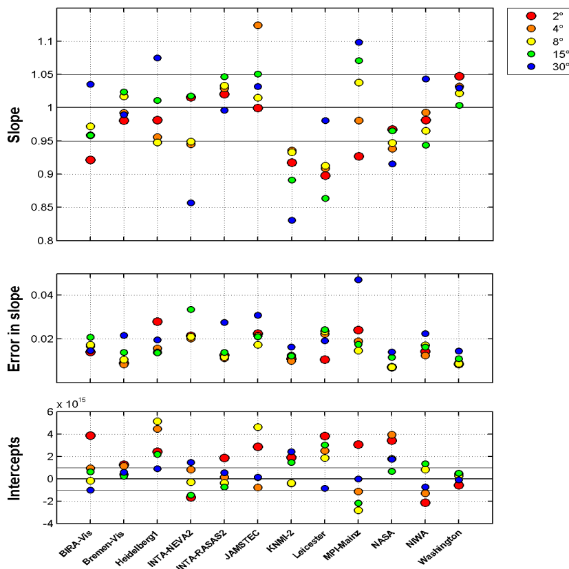
Fig. 8. Straight-line slopes and their errors of NO 2 slant columns against those of the reference data set, for each instrument at visible wavelengths, for clear sunny mornings only. Colours refer to elevation angles shown top right. Note the similarity to Fig. 6 in differences from unity slope for many instruments, but with larger scatter and errors because the number of data points is much smaller.
