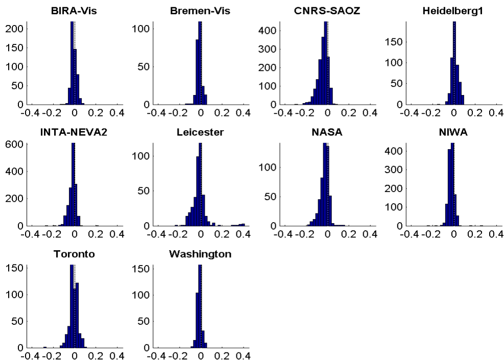
Fig. 17. Histograms of the differences between zenith-sky results from each instrument and results interpolated from INTA-RASAS2. The histograms are for the whole campaign, and are normalised by the difference between the mean INTA-RASAS2 slope and the mean of all instruments. If both INTA-RASAS2 and the other instrument were of high standard, one would expect a narrow and symmetric histogram, though not necessarily symmetric about zero. The fact that several histograms are narrow and symmetric strongly suggests that they and INTA-RASAS2 are both of high standard.
