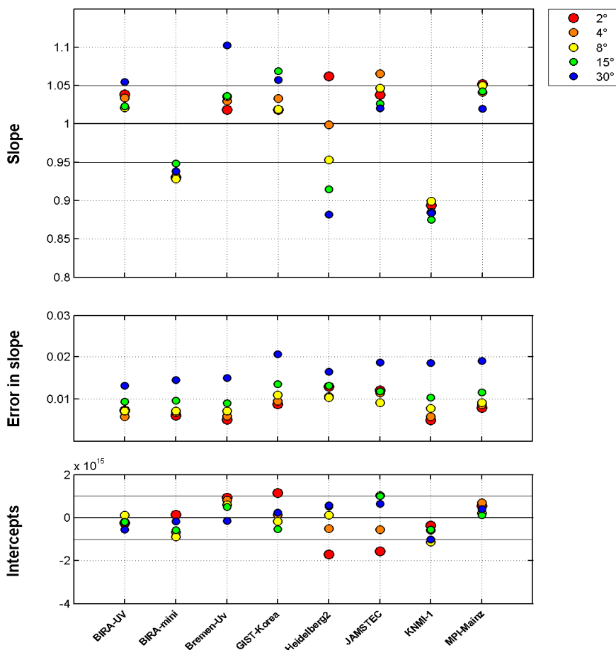
Fig. 10. Straight-line slopes and their errors of NO 2 slant columns against those of the reference data set, for each instrument at UV wavelengths and for the whole campaign. Colours refer to elevation angles shown top right.
