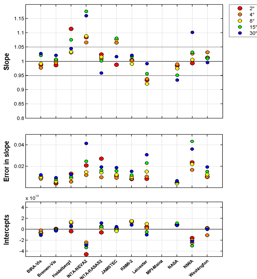
Fig. 7. Straight-line slopes and their errors of O 4 slant columns against those of the reference data set, for each instrument at visible wavelengths and for the whole campaign. Colours refer to elevation angles shown top right. MPI-Mainz used a non-standard wavelength range for analysis, which did not produce an O 4 amount.
