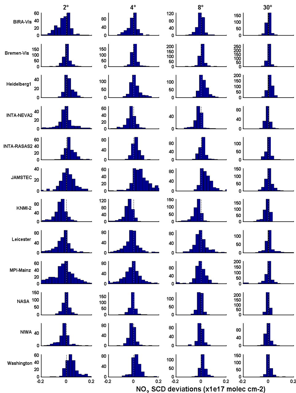
Fig. 9. Histograms of the absolute deviations of visible measurements from the reference visible data set, for the whole campaign.
