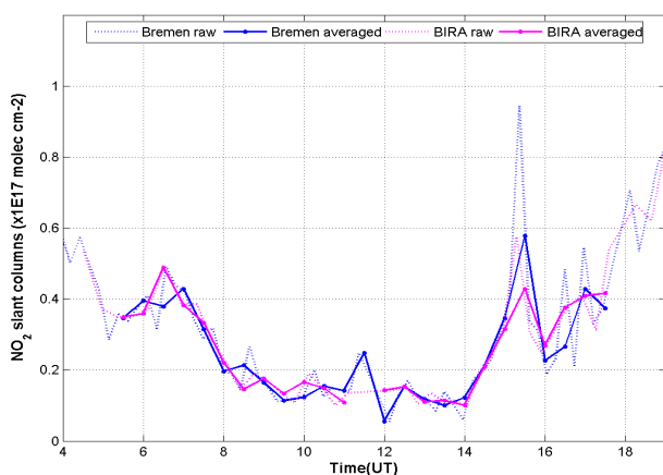
Fig. 4. Comparison of raw and 30-min averaged slant columns of NO 2 measured by Bremen and BIRA, on 19 June 2009 at elevation 15°. These are weighted averages, using as a weight the inverse square of the error of each data point given by its spectral fit. Measurements by BIRA are missing near local noon because BIRA investigators chose a longer period of measurements at 90° elevation in order to increase the chances of a cloud-free reference spectrum for the day.
