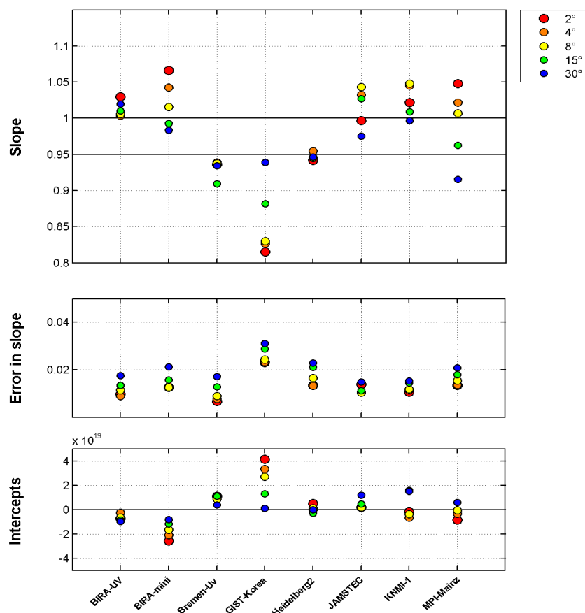
Fig. 11. Straight-line slopes and their errors of O 4 slant columns against those of the reference data set, for each instrument at UV wavelengths and for the whole campaign. Colours refer to elevation angles shown top right.
