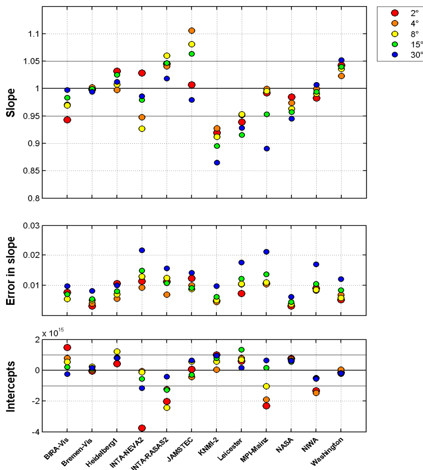
Fig. 6. Straight-line slopes and their standard errors of NO 2 slant columns against those of the reference data set, for each instrument at visible wavelengths and for the whole campaign. Colours refer to elevation angles shown top right. Note that MPI-Mainz used a non-standard wavelength range for spectral analysis because of the limited range of the instrument (see Table 1).
