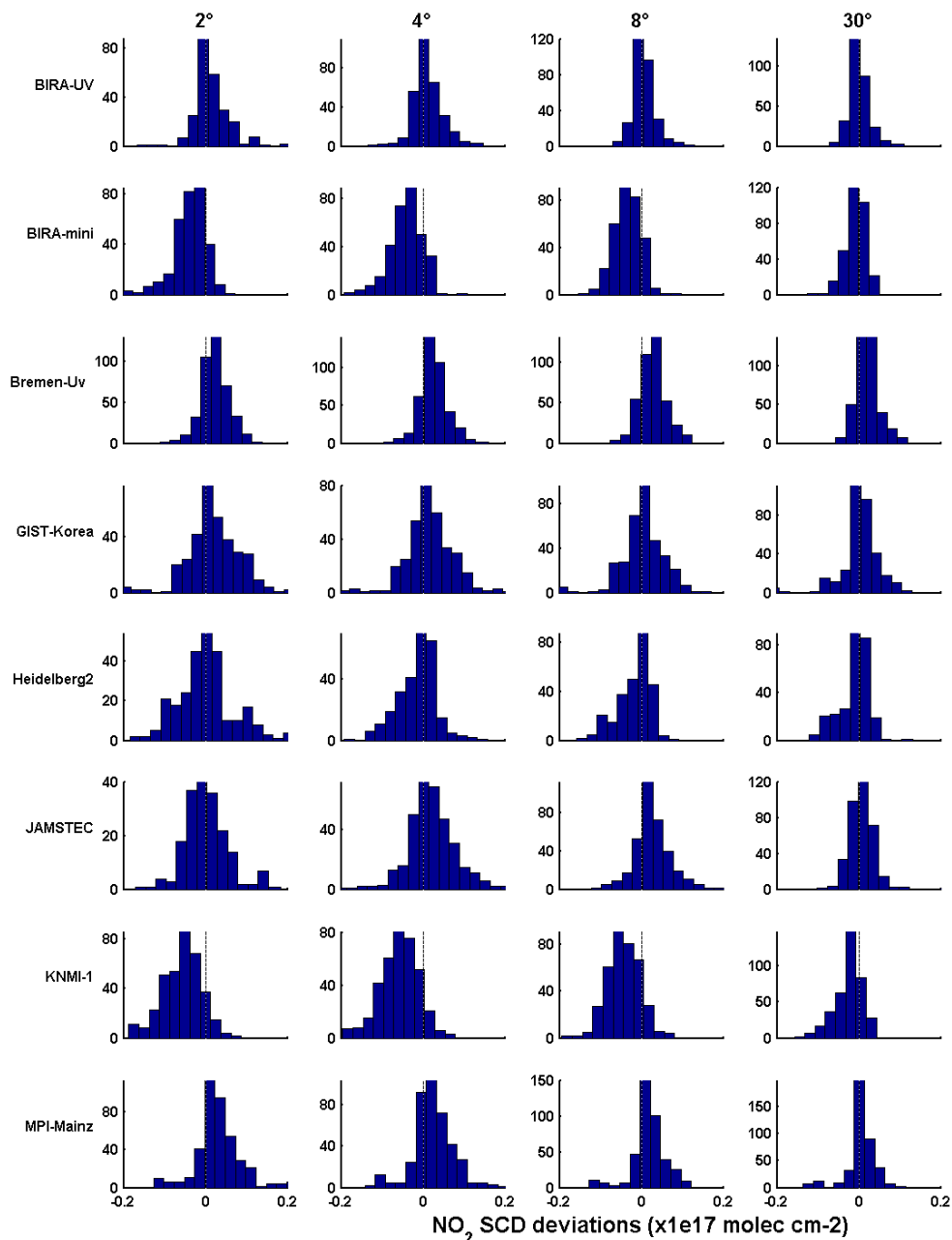
Fig. 12. Histograms of the absolute deviations of UV measurements from the reference UV data set, for the whole campaign.
